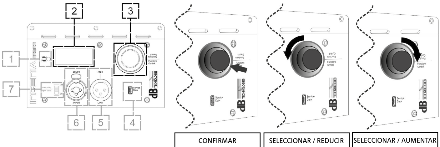
Push rotary encoder
